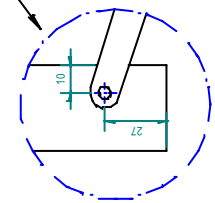
Thrust bar anchoring to dishwasher details (Make a hole Ø6)
