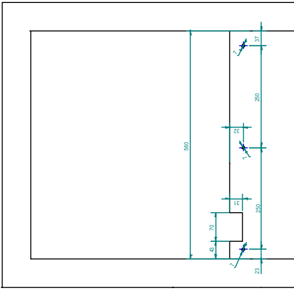
Exit of raised appliance (left version)
